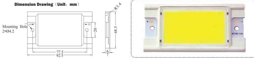
Dimension Drawing (Unit: mm)
