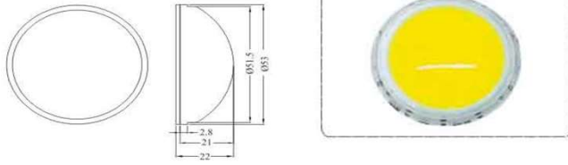
Dimension Drawing (Unit: mm)
